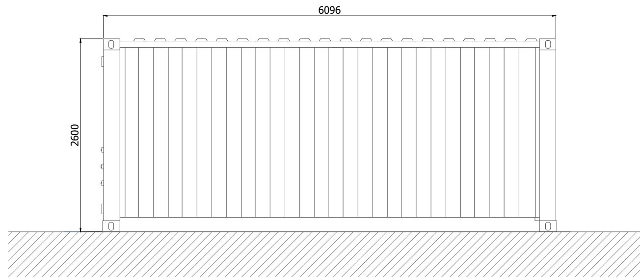
FRONT ELEVATION
