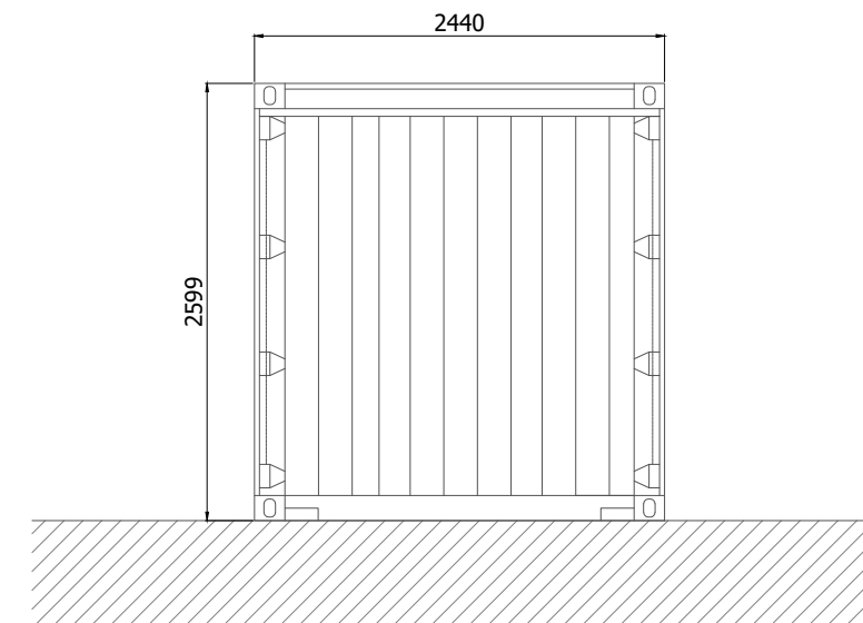
SIDE ELEVATION
