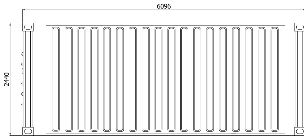
ROOF PLAN
